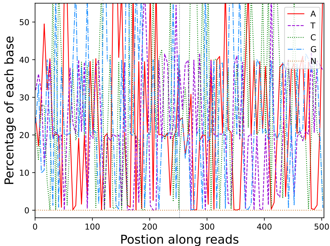
Base percentage along reads (R10504)
